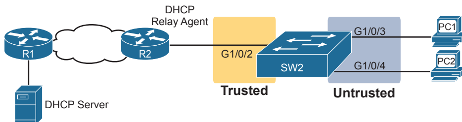
Figure 8-15 Sample Network Used in ARP Inspection Configuration Examples
