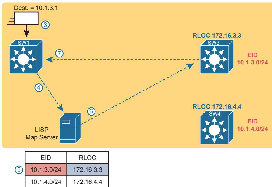
Figure 17-9 Ingress Tunnel Router SW1 Discovers Egress Tunnel Router SW3 Using LISP
