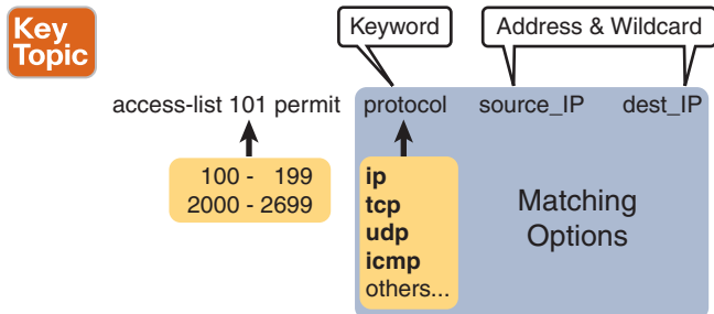
Figure 3-3 Extended ACL Syntax, with Required Fields
