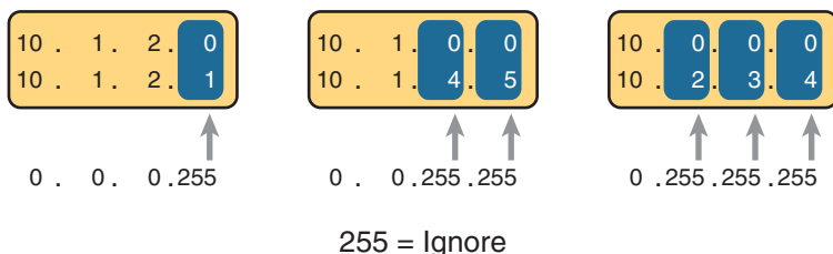
Figure 2-6 Logic for WC Masks 0.0.0.255, 0.0.255.255, and 0.255.255.255
