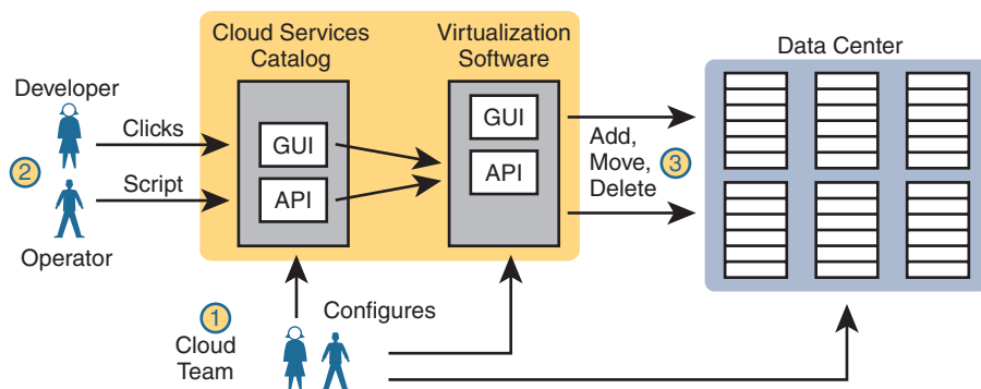
Figure 15-7 Basic Private Cloud Workflow to Create One VM
