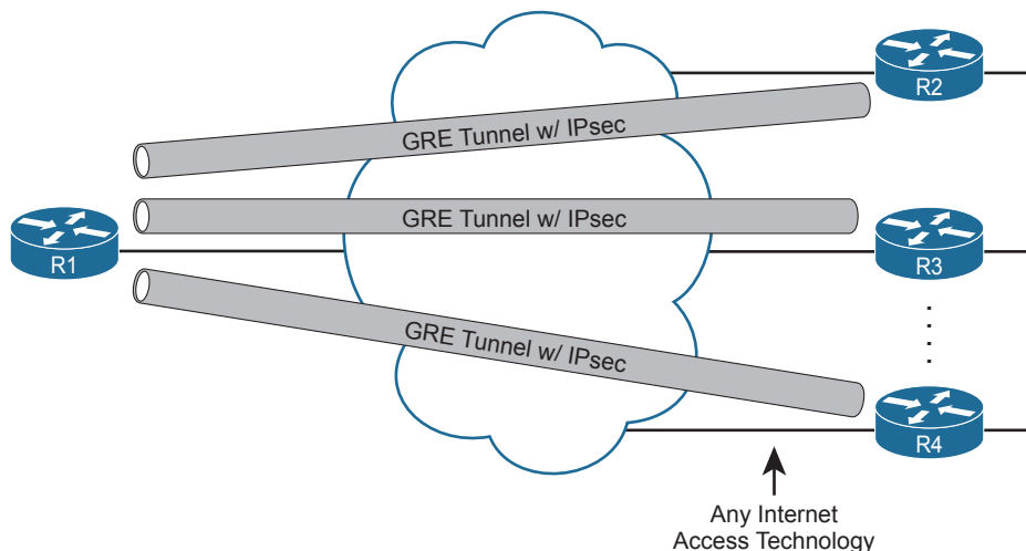
Figure 14-22 Site-to-Site VPN Tunnels with GRE and IPsec
