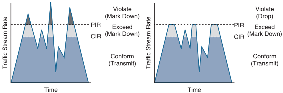
Figure 14-15 Two-Rate Three-Color Marker/Policer Token Bucket Algorithm
