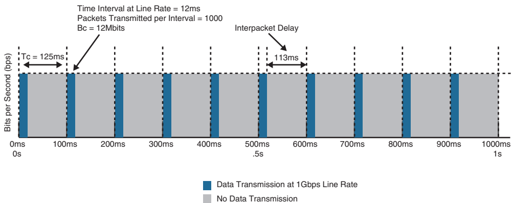
Figure 14-11 Token Bucket Operation
