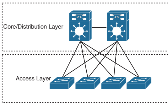
Figure 22-2 Modular Design Scalability
