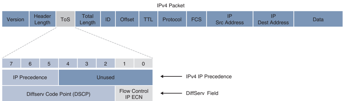
Figure 14-3 IPv4 ToS/DiffServ Field
