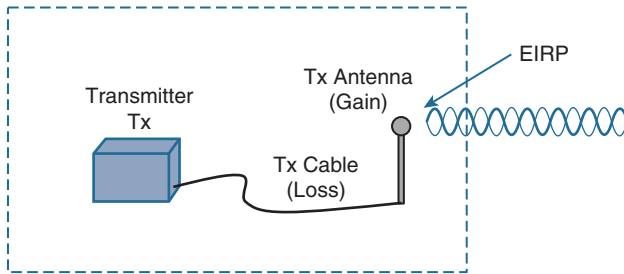
Figure 17-20 Calculating EIRP
