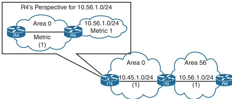
Figure 9-10 Visualization of the 10.56.1.0/24 Type 3 LSA from Area 0
