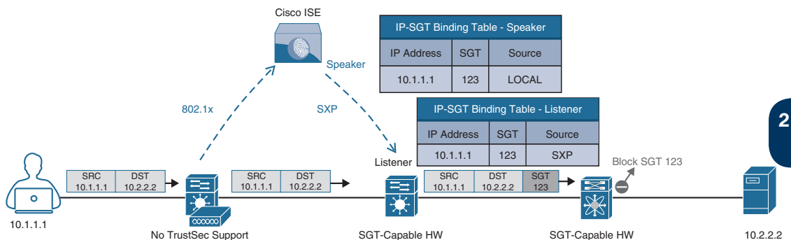
Figure 25-14 TrustSec Enforcement with SGACL
