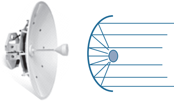
Figure 18-25 Cisco Parabolic Dish Antenna
