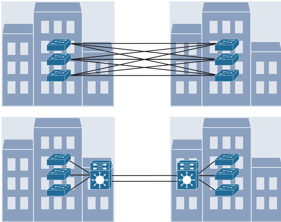
Figure 22-5 Distribution Layer Reducing Fiber-Optic Runs
