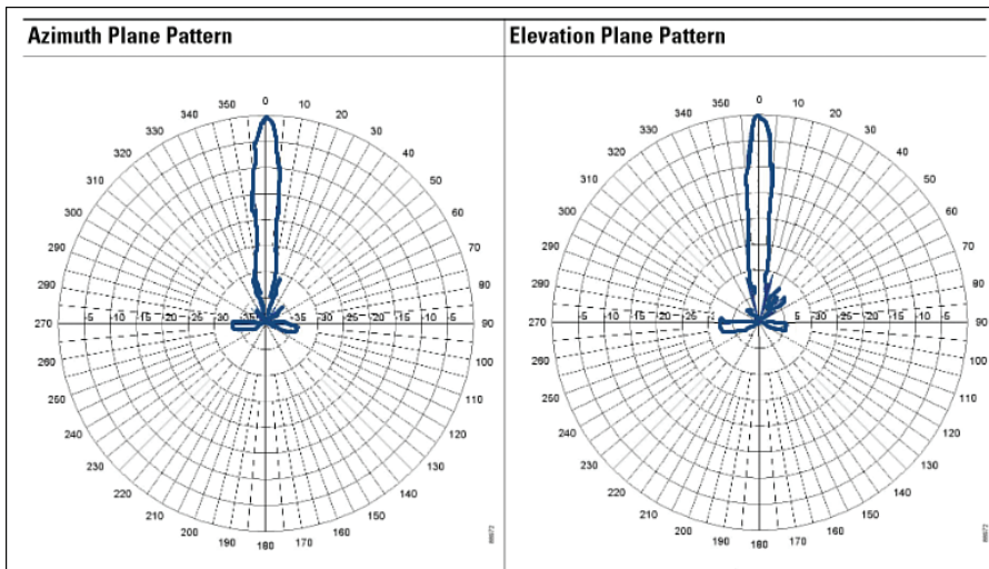
Figure 18-26 E and H Radiation Patterns for a Parabolic Dish Antenna
