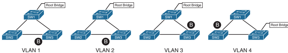
Figure 4-2 Per-VLAN Spanning Tree (PVST) Topologies
