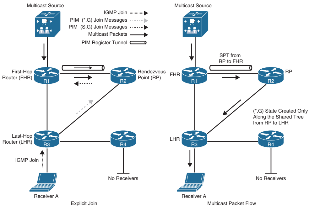
Figure 13-17 PIM-SM Multicast Distribution Tree Building
