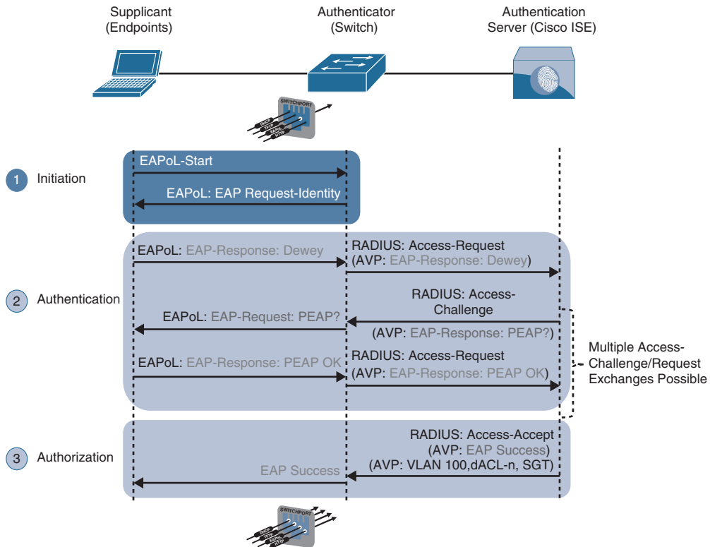
Figure 25-7 Successful 802.1x Authentication Process Flow
