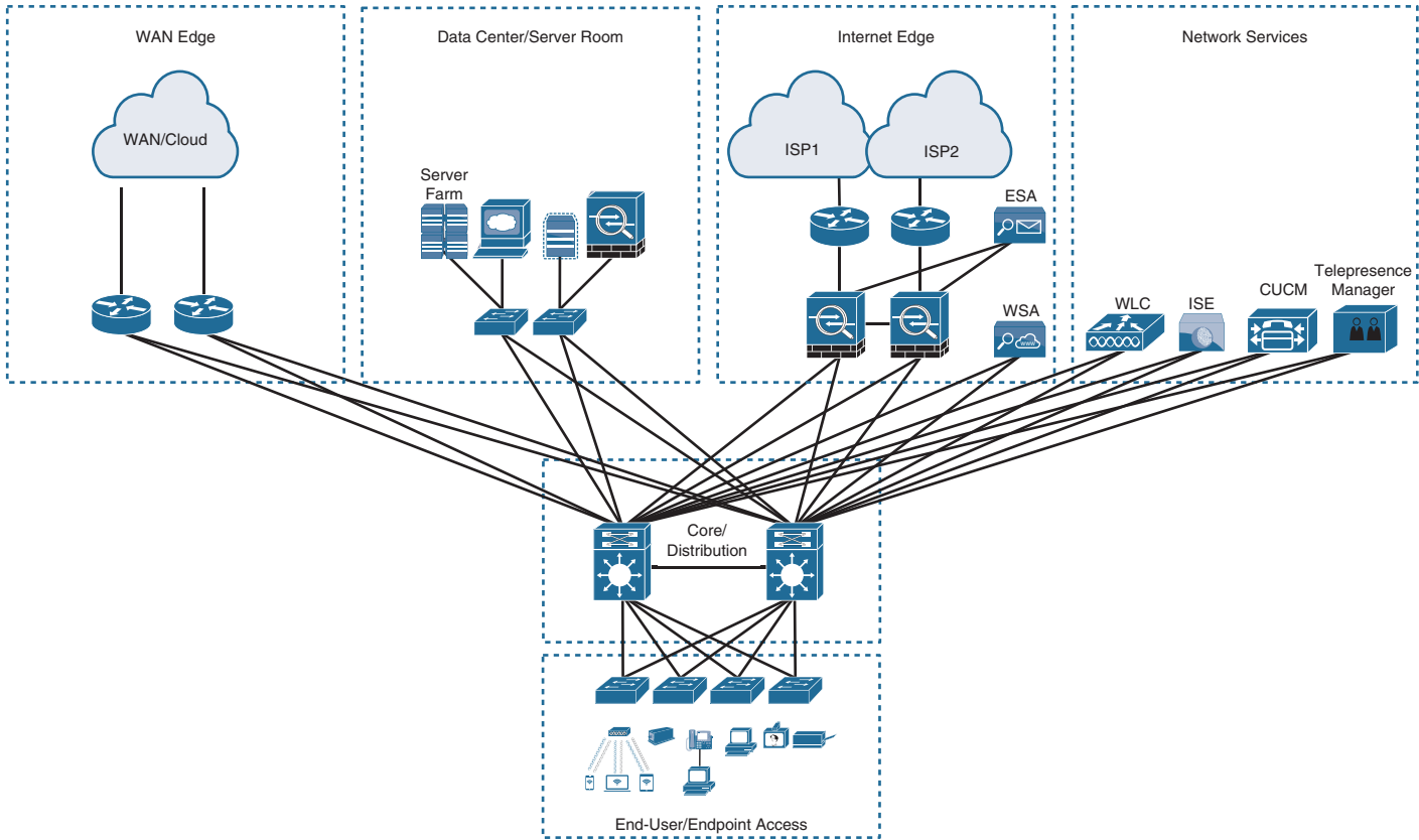
Figure 22-7 Two-Tier/Collapsed Core Design
