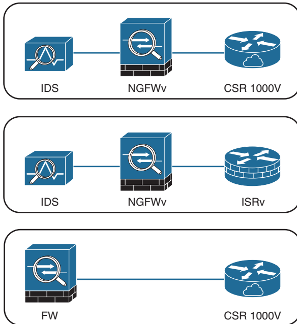
Figure 27-8 Service Chaining
