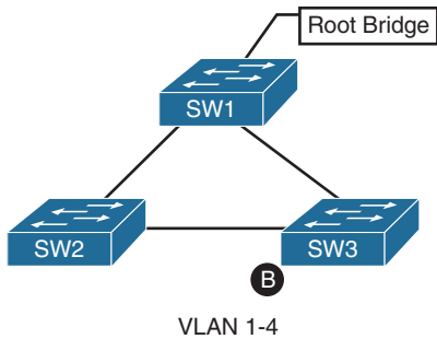
Figure 4-1 Common Spanning Tree Instance (CST) Topology
