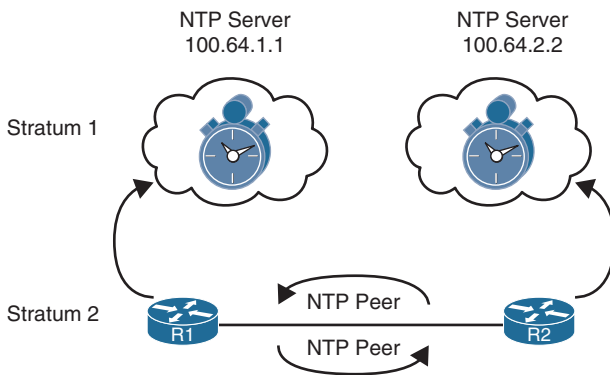
Figure 15-3 NTP Stratum
