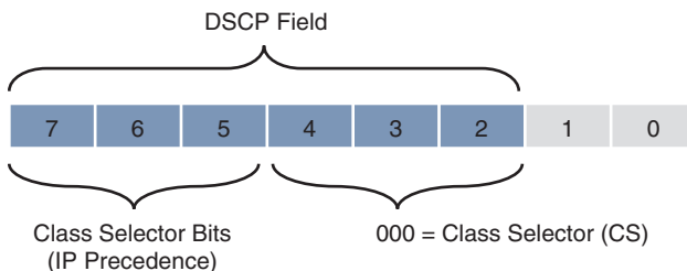
Figure 14-4 Class Selector (CS) PHB
