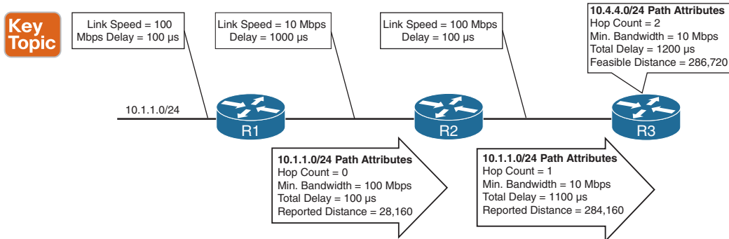
Figure 7-7 EIGRP Attribute Propagation
