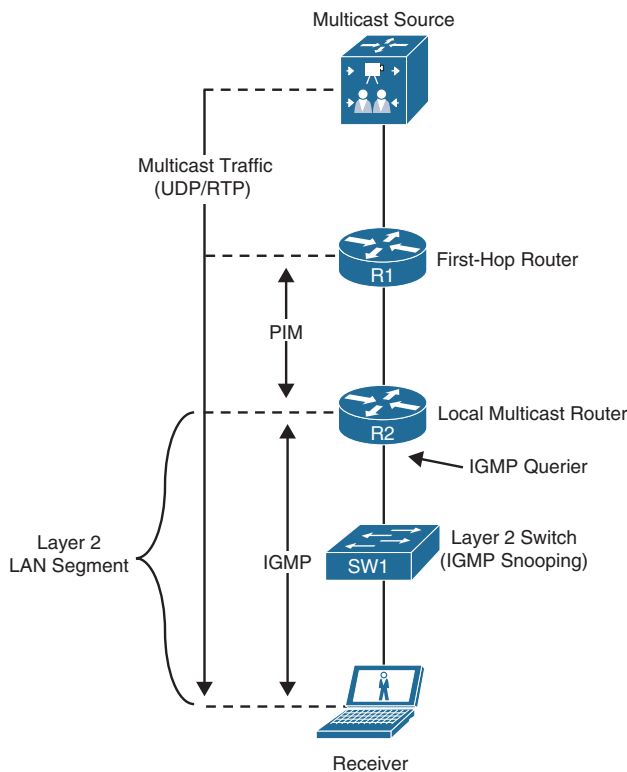
Figure 13-1 Multicast Architecture
