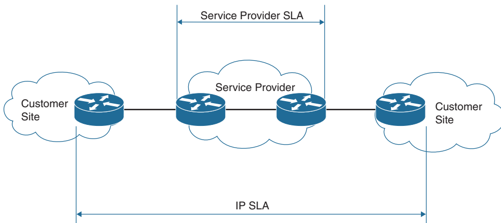
Figure 24-5 IP SLA and Typical Service Provider SLA
