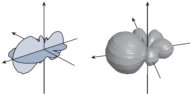
Figure 18-24 Yagi Antenna Radiation Pattern in Three Dimensions
