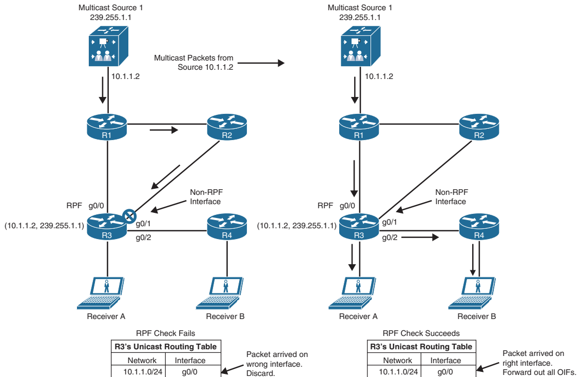
Figure 13-19 RPF Check
