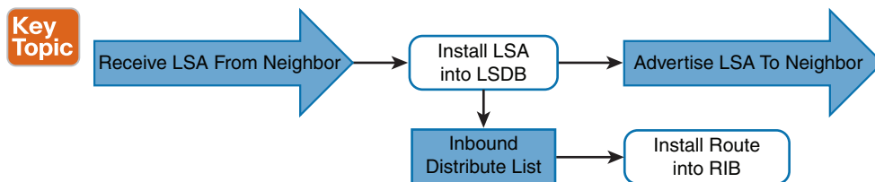
Figure 9-25 OSPF Distribute List Filtering Logic
