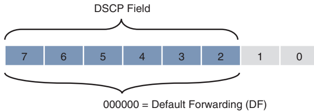
Figure 14-5 Default Forwarding (DF) PHB
