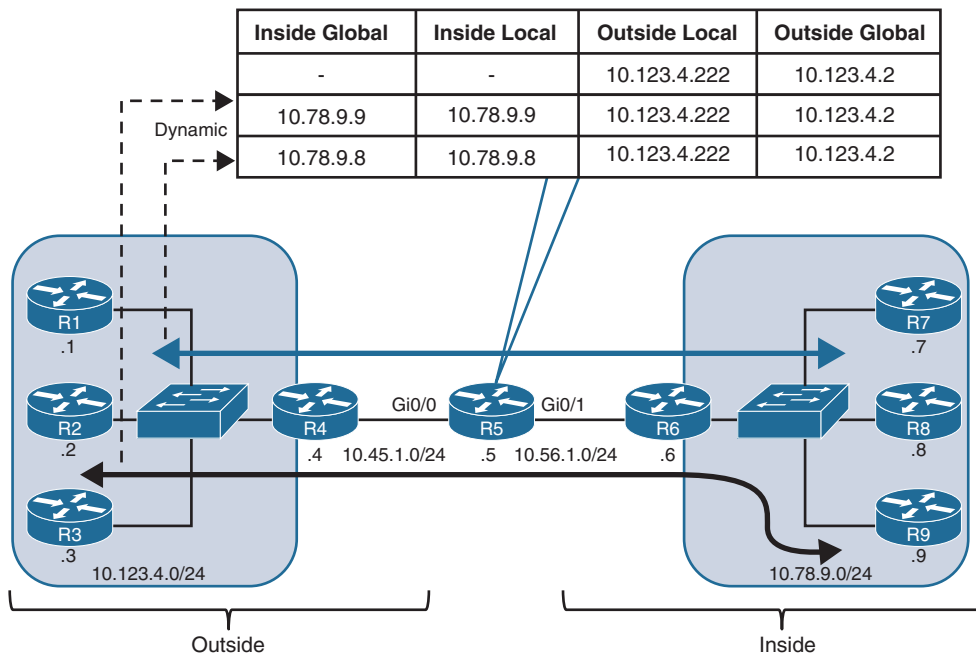
Figure 15-9 Outside Static NAT Topology for R2 as 10.123.4.222
