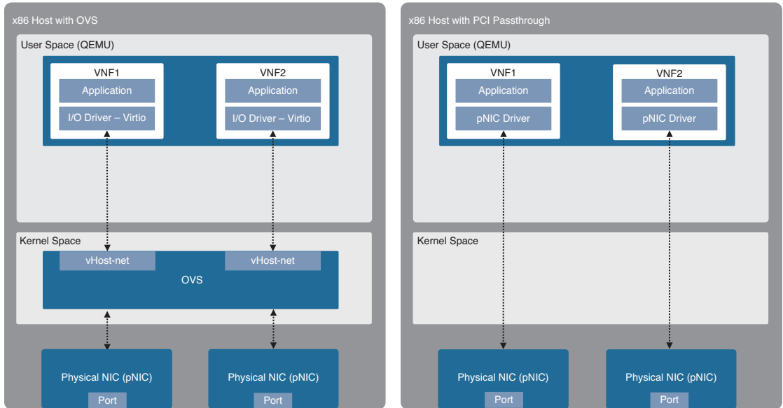
Figure 27-12 Standard OVS and PCI Passthrough
