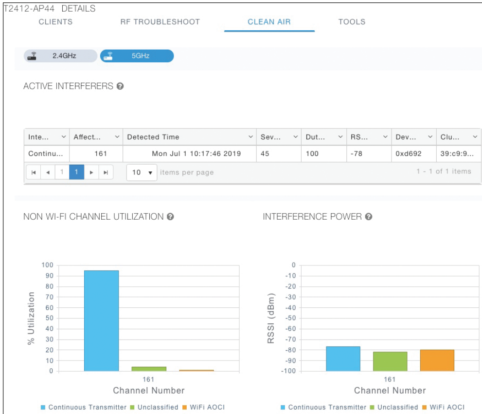
Figure 21-17 Displaying Information
