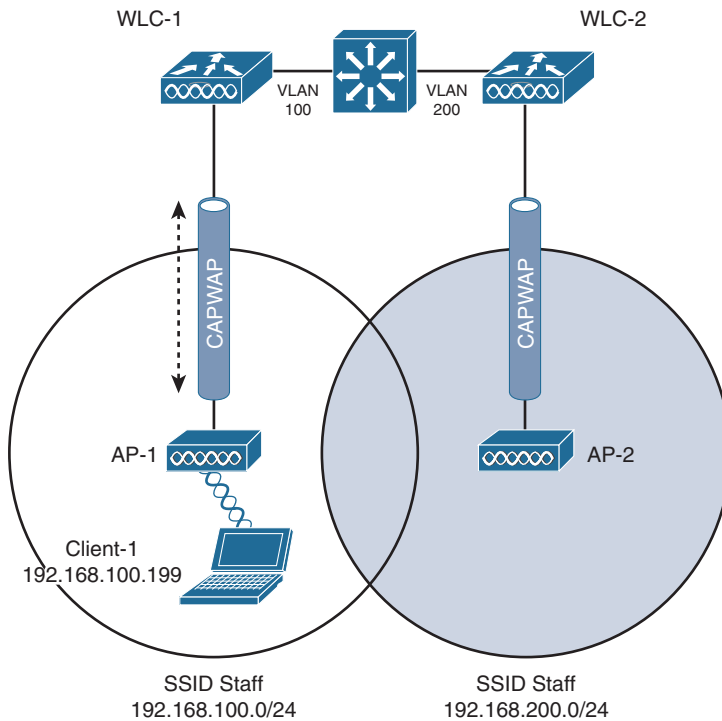
Figure 19-8 Before a Layer 3 Intercontroller Roam
