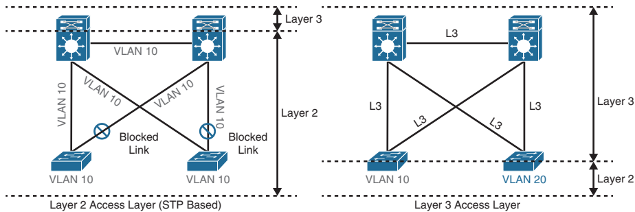
Figure 22-10 Layer 2 Access Layer and Layer 3 Access Layer
