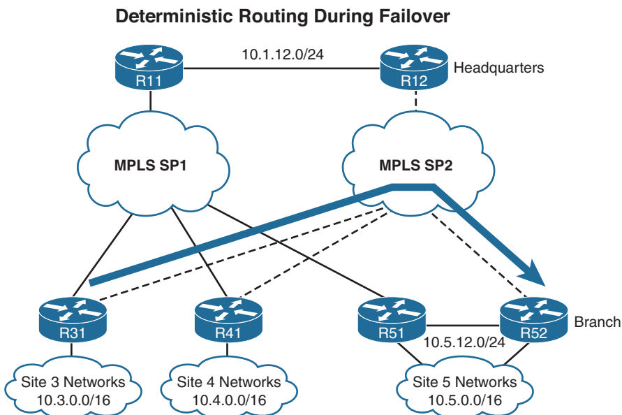
Figure 12-3 Deterministic Routing
