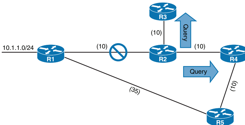
Figure 7-14 EIGRP Convergence Topology
