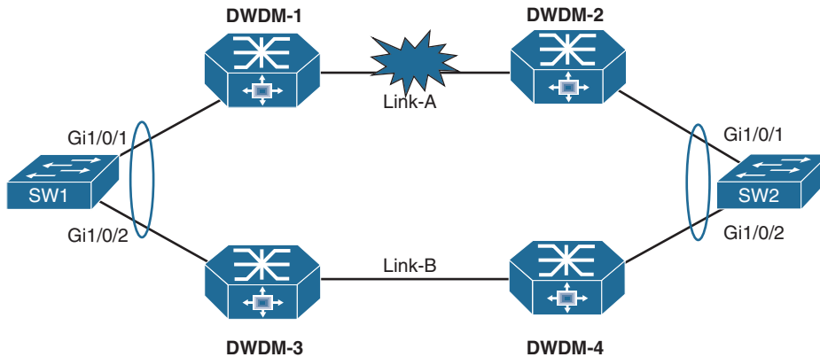
Figure 5-4 Port-Channel Link-State Propagation and Detection
