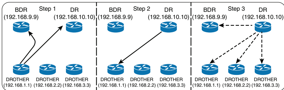
Figure 8-6 Network Prefix Advertisement with DR Segments
