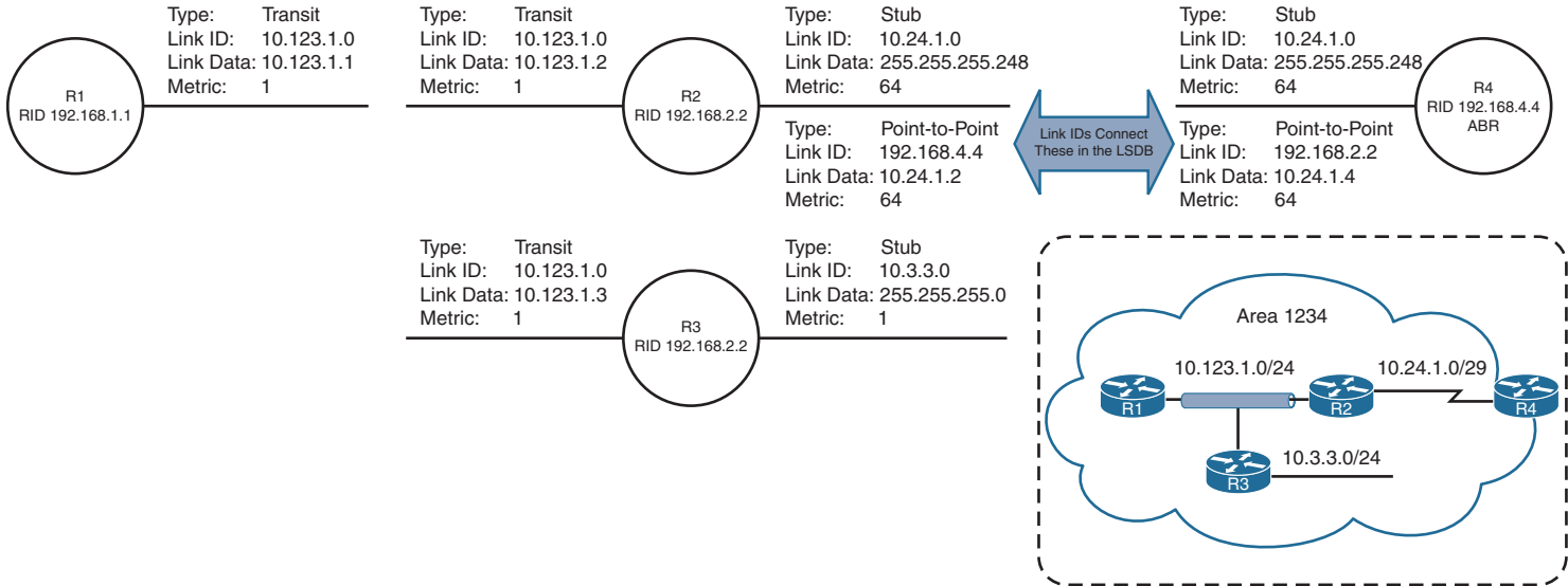
Figure 9-7 Visualization of Type 1 LSAs
