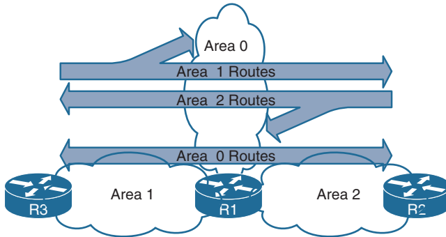
Figure 9-2 Successful Route Advertisement Between Areas
