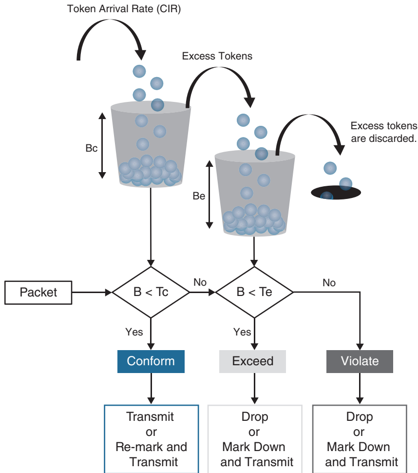
Figure 14-14 Single-Rate Three-Color Marker/Policer Token Bucket Algorithm
