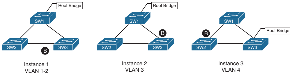
Figure 4-3 MST Topologies
