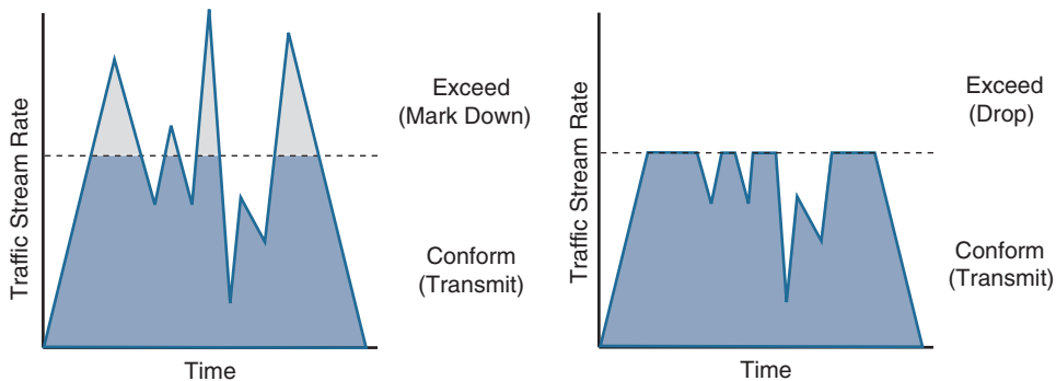
Figure 14-12 Single-Rate Two-Color Marker/Policer
