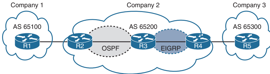
Figure 11-3 AS 65200 Providing Transit Connectivity
