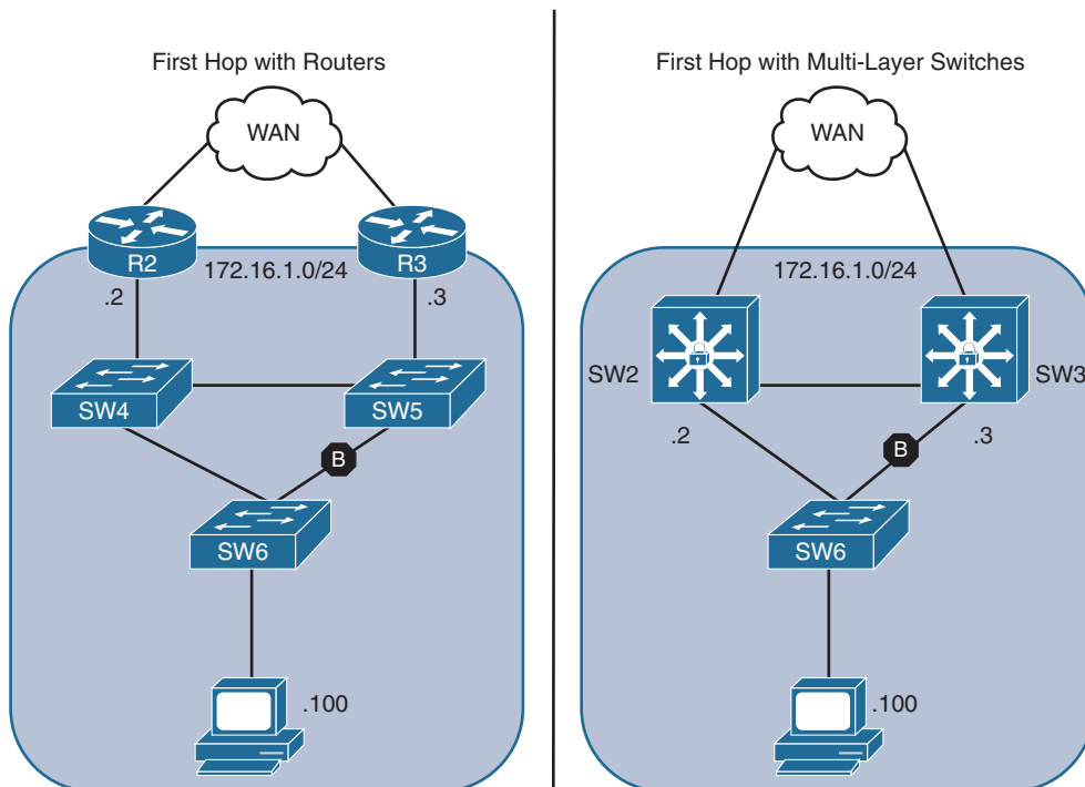
Figure 15-4 Resiliency with Redundancy with Layer 2 and Layer 3 Devices
