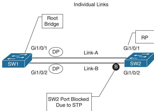
Figure 5-2 Multiple Links with STP
