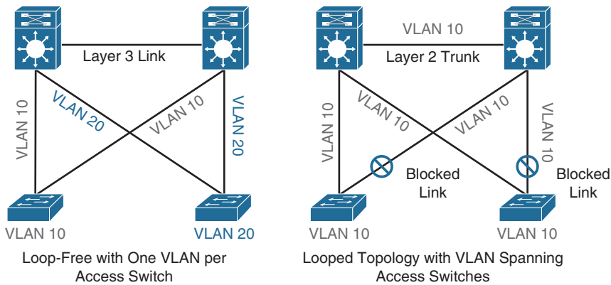
Figure 22-9 Loop-Free Topology and Looped Topology
