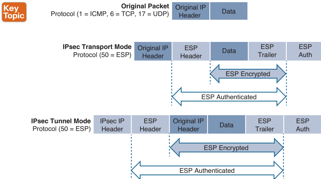
Figure 16-3 IPsec Transport and Tunnel Encapsulation
