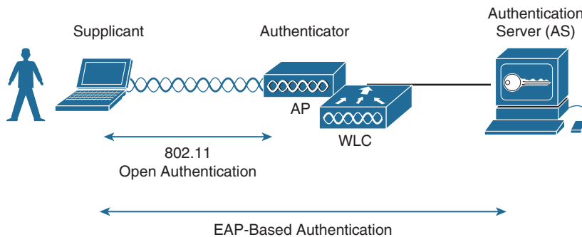
Figure 20-8 802.1x Client Authentication Roles
