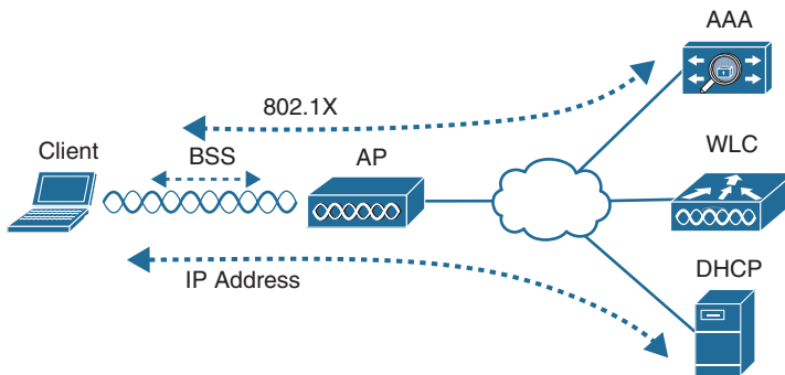
Figure 21-1 Conditions for a Successful Wireless Association
