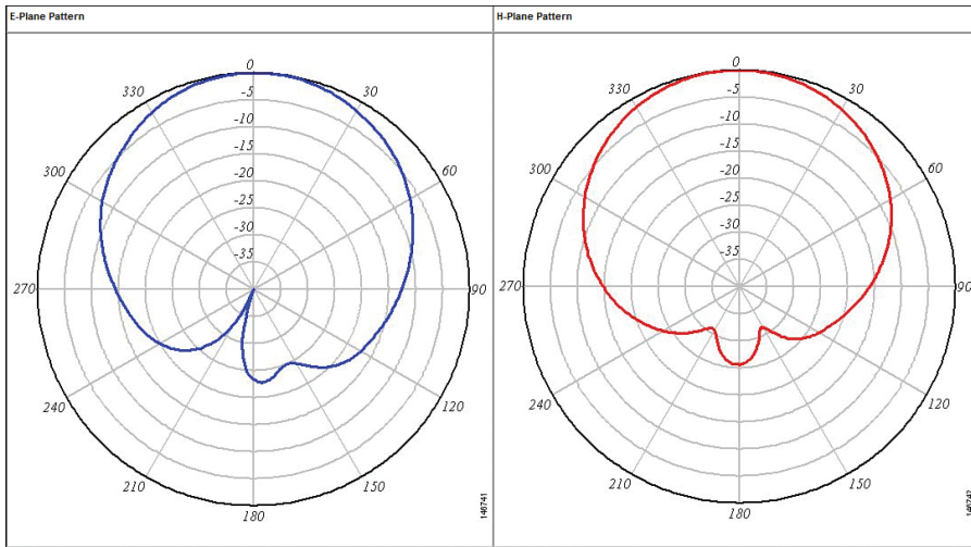
Figure 18-20 E and H Radiation Patterns for a Typical Patch Antenna
