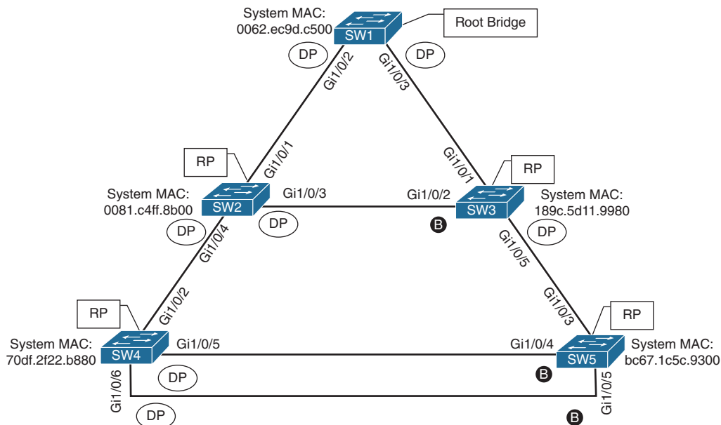
Figure 3-1 STP Topology for Tuning
