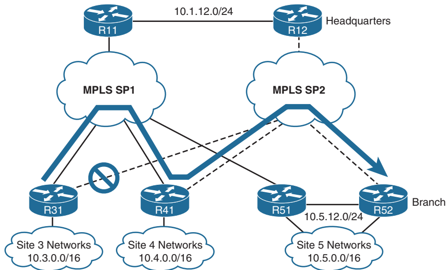
Figure 12-4 Nondeterministic Routing During Failover
