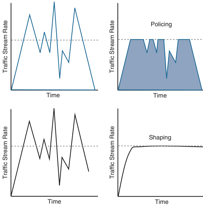
Figure 14-9 Policing Versus Shaping
