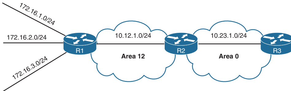
Figure 9-21 OSPF Interarea Summarization Example
