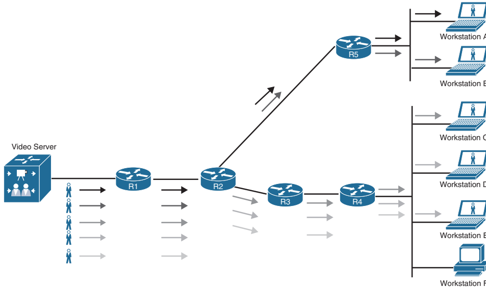
Figure 13-2 Unicast Video Feed
