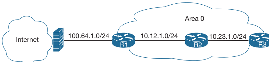
Figure 8-8 Default Route Topology
