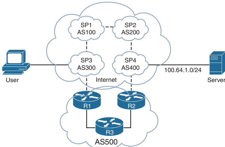
Figure 12-2 Enterprise Transit Routing
