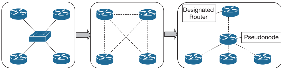
Figure 8-5 OSPF DR Concept
