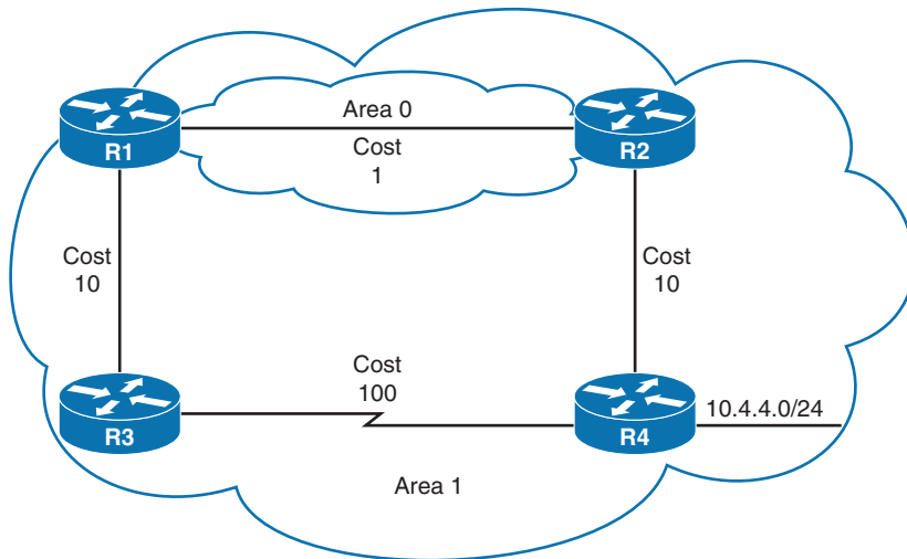
Figure 9-14 Intra-Area Routes over Interarea Routes
