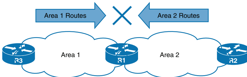
Figure 9-1 Failed Route Advertisement Between Areas
