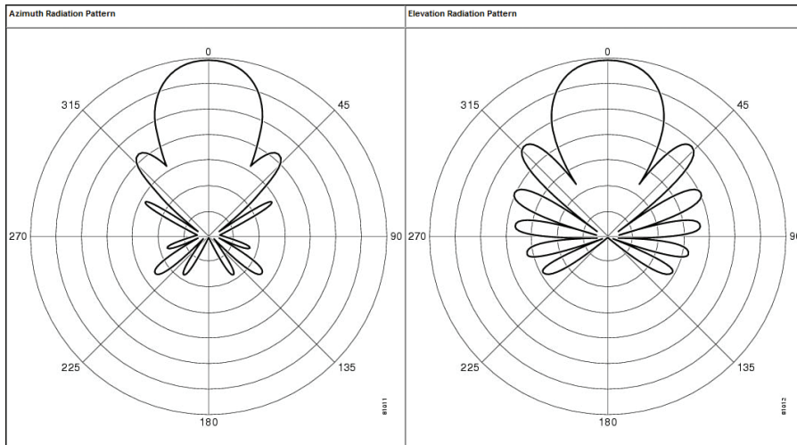
Figure 18-23 E and H Radiation Patterns for a Typical Yagi Antenna
