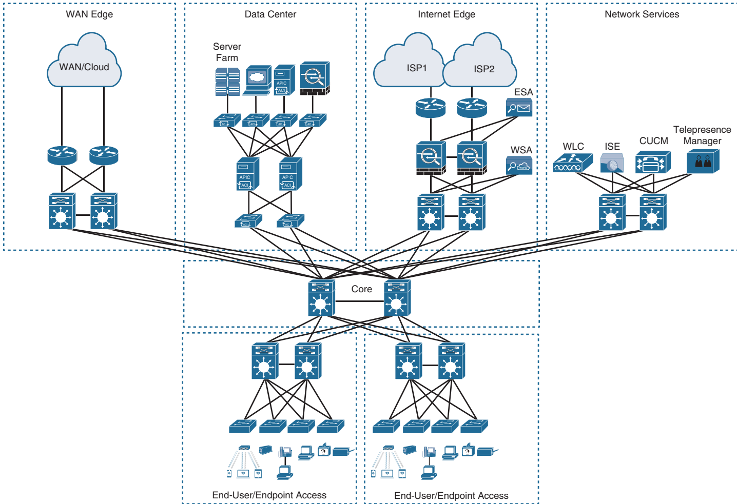
Figure 22-8 Three-Tier Design
