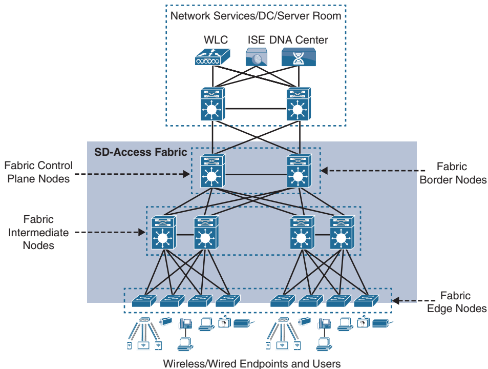
Figure 23-6 SD-Access Fabric Roles
