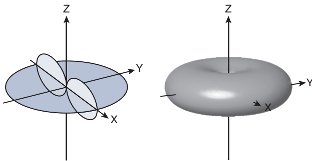
Figure 18-16 Dipole Radiation Pattern in Three Dimensions
