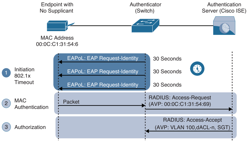
Figure 25-8 Successful MAB Authentication Process Flow
