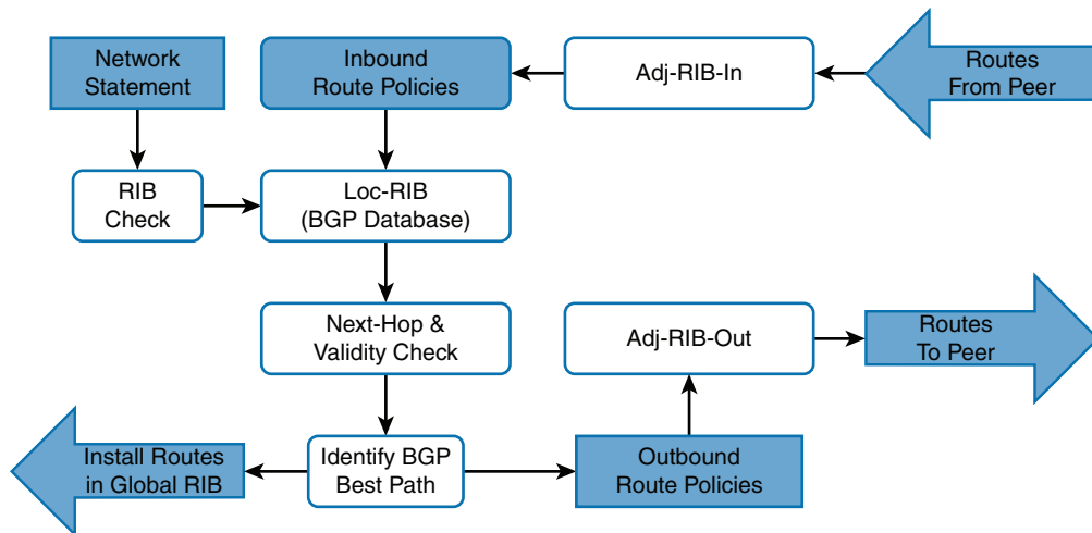
Figure 12-9 BGP Route Policy Processing
