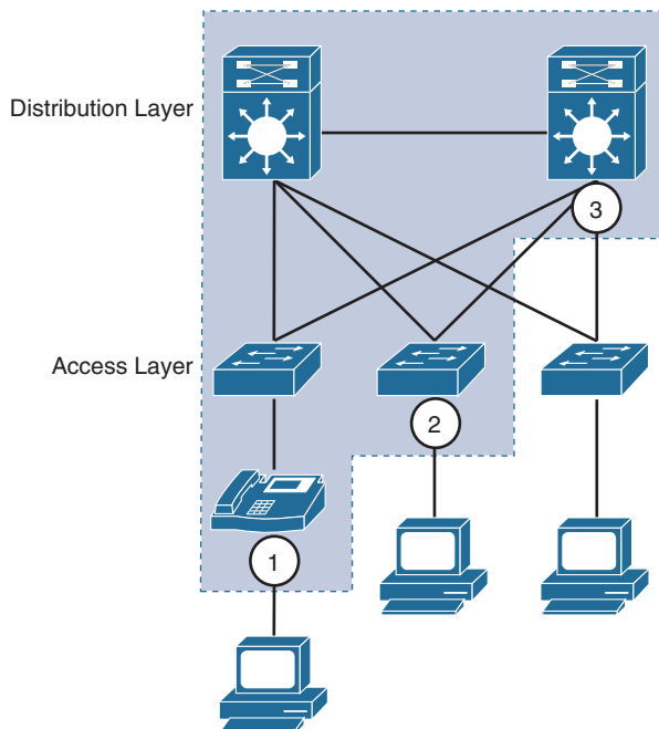
Figure 14-7 Trust Boundaries
