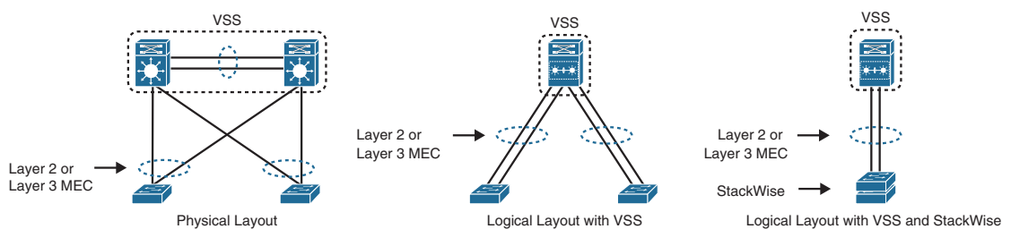
Figure 22-11 Simplified Campus Design with VSS and StackWise
