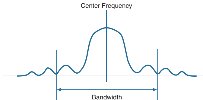
Figure 17-8 Signal Bandwidth
