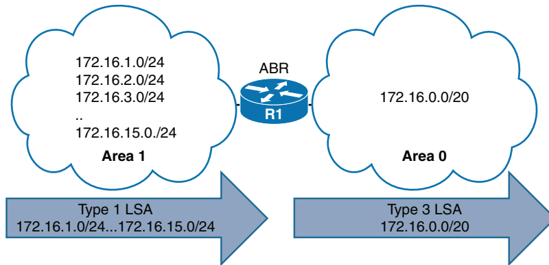
Figure 9-19 OSPF Interarea Summarization
