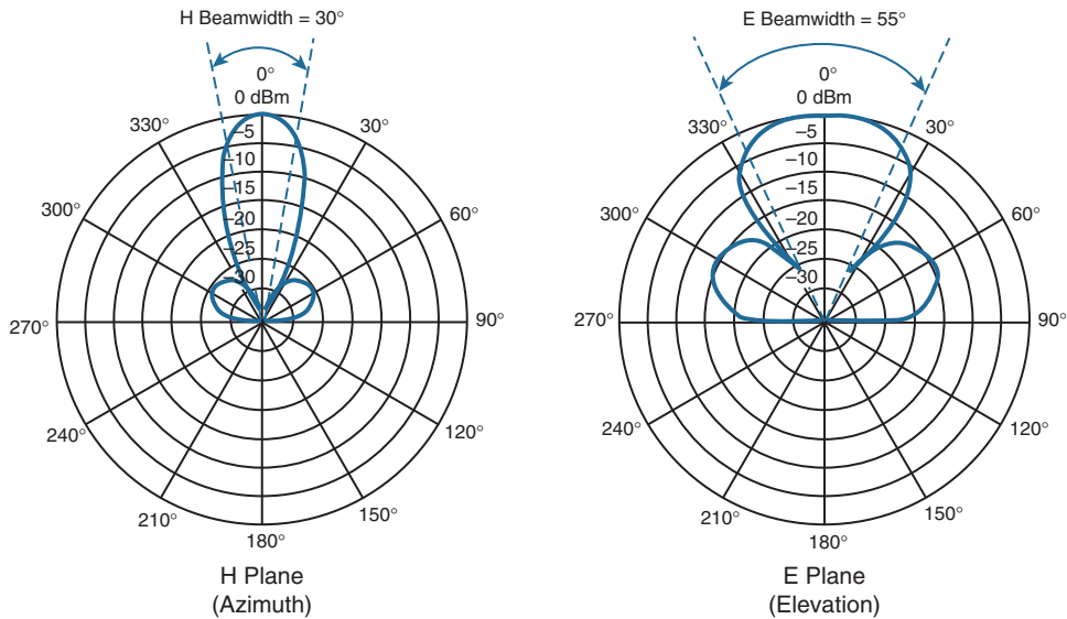
Figure 18-12 Example of Antenna Beamwidth Measurement
