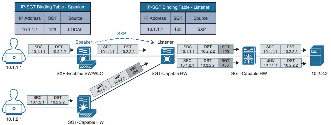
Figure 25-12 Inline Tagging and SXP Propagation
