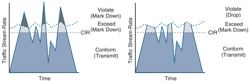
Figure 14-13 Single-Rate Three-Color Marker/Policer
