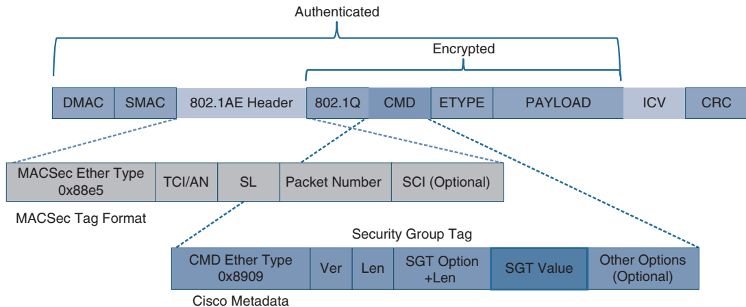
Figure 25-18 MACsec Ethernet Frame with SGT
