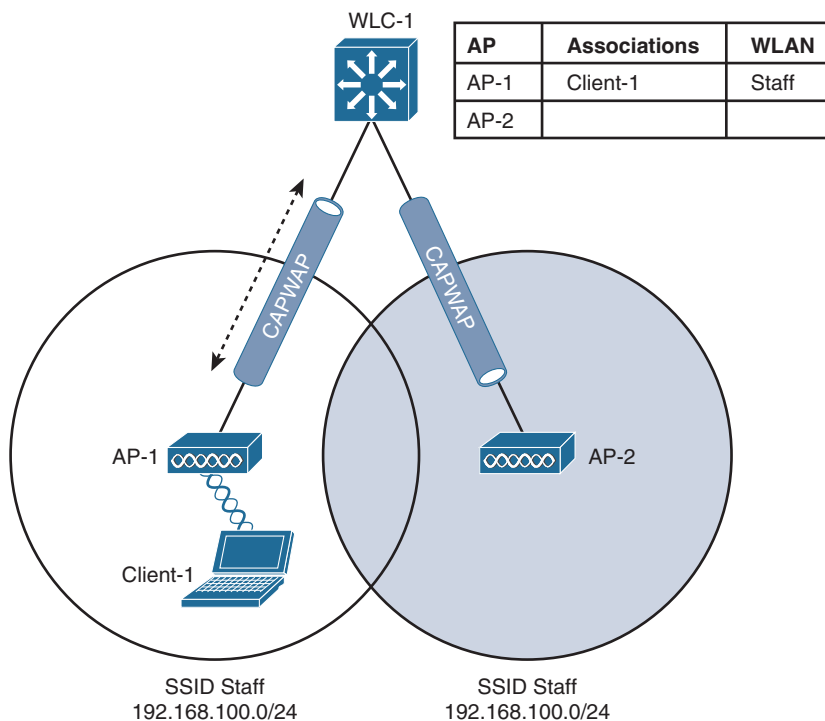
Figure 19-4 Cisco Wireless Network Before an Intracontroller Roam
