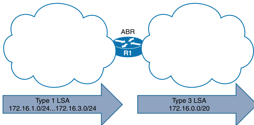
Figure 9-20 Interarea Summarization Metric
