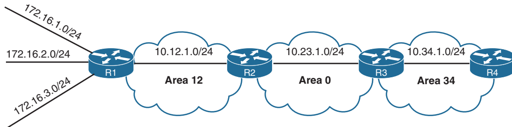
Figure 9-22 Expanded Topology for Filtering Routes
