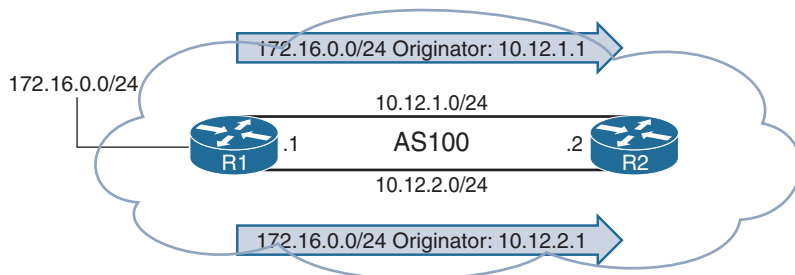
Figure 12-13 Lowest IP Address
