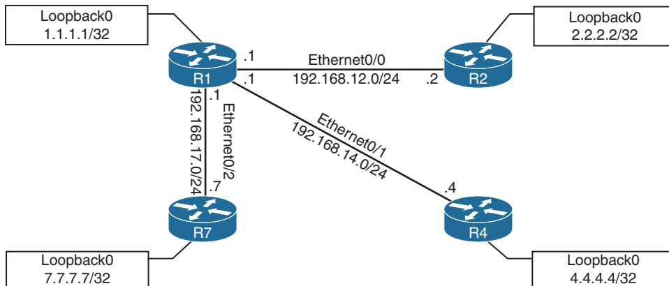
Figure 24-2 Debugging Topology
