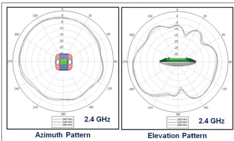
Figure 18-18 E and H Radiation Patterns for a Typical Integrated Omnidirectional Antenna
