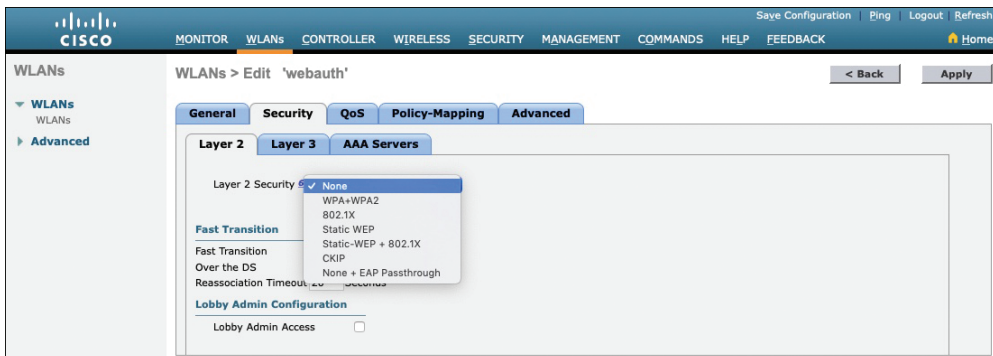
Figure 20-18 Configuring Open Authentication for WebAuth
