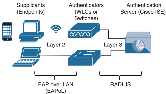
Figure 25-6 802.1x Roles and Components
