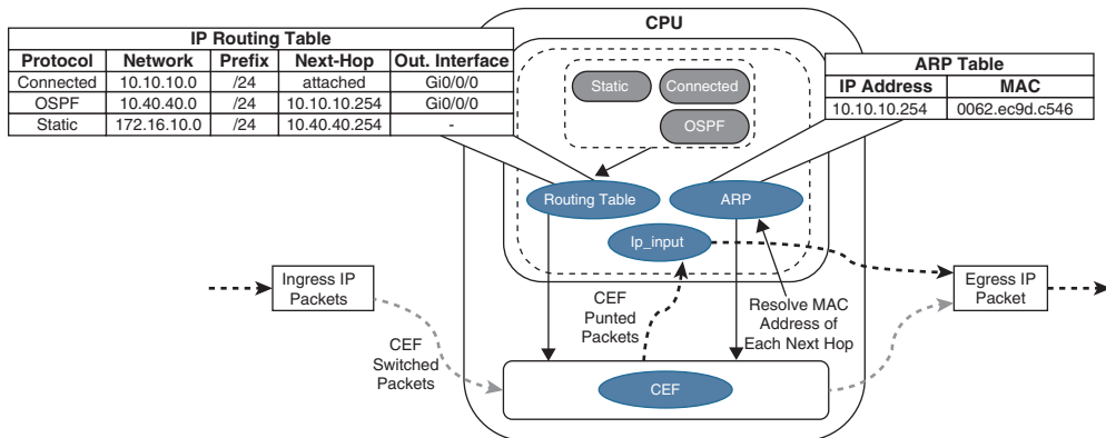
Figure 1-6 Process Switching
