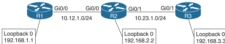
Figure 15-5 Object Tracking
