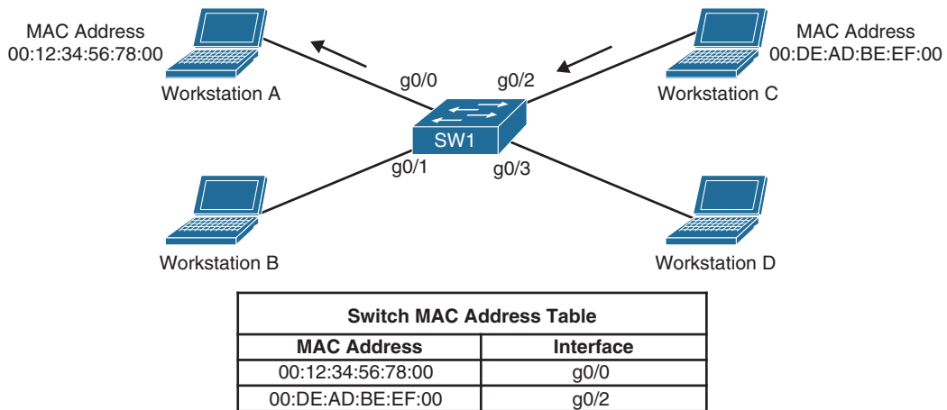
Figure 13-9 Known Destination Is Not Flooded
