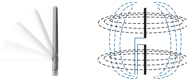
Figure 18-14 Cisco Dipole Antenna
