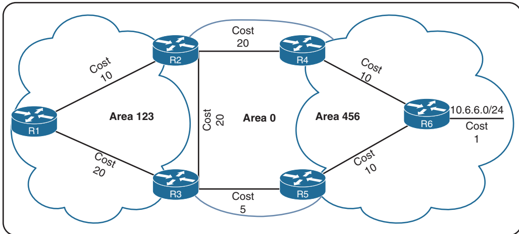
Figure 9-15 Interarea Route Selection
