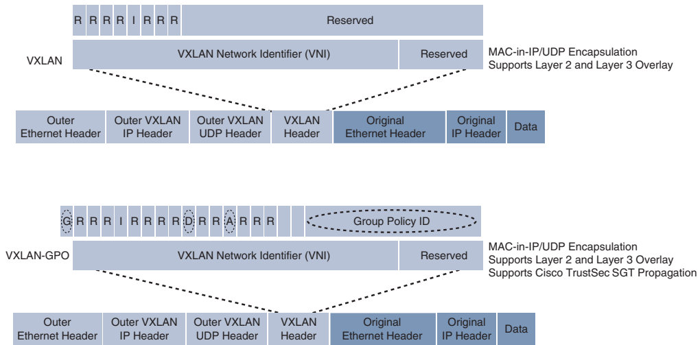
Figure 23-5 VXLAN and VXLAN-GPO Packet Format Comparison
