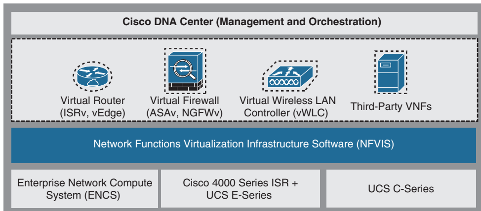
Figure 27-14 Enterprise NFV Solution Main Components
