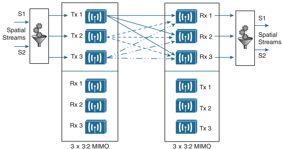
Figure 17-29 Spatial Multiplexing Between Two 3×3:2 MIMO Devices
