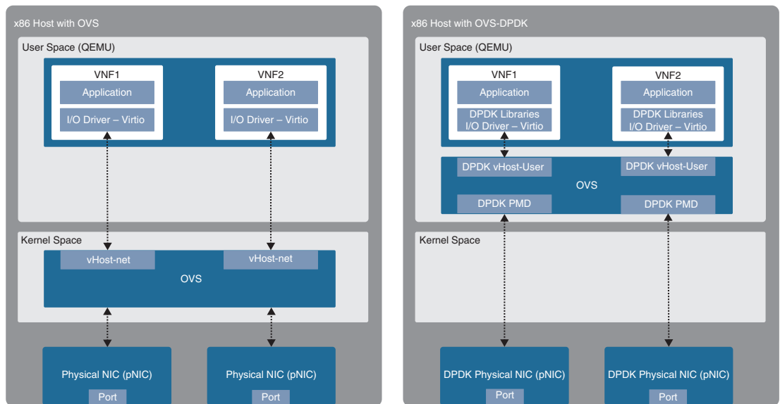
Figure 27-11 Standard OVS and OVS-DPDK
