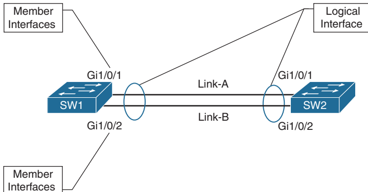
Figure 5-3 EtherChannel Components
