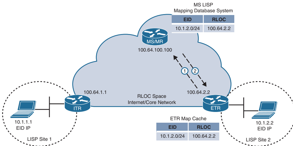
Figure 16-8 Map Registration and Notification
