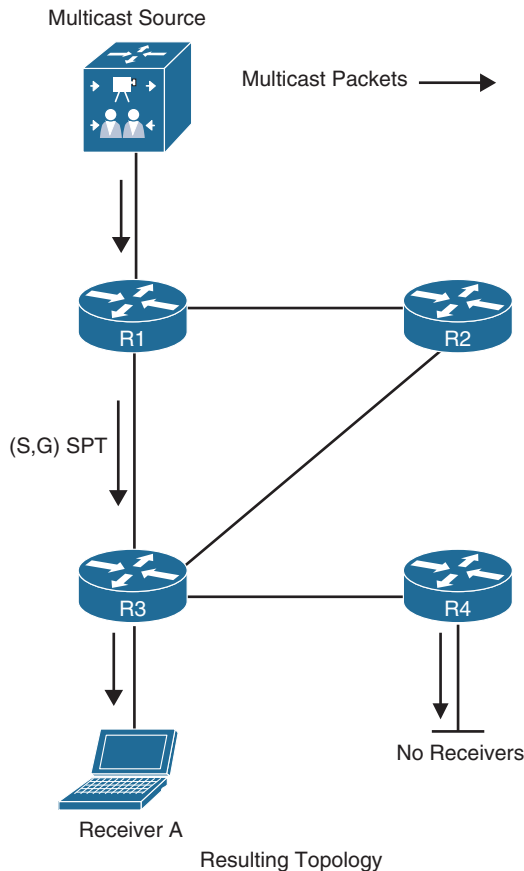
Figure 13-16 PIM-DM Resulting Topology After Pruning
