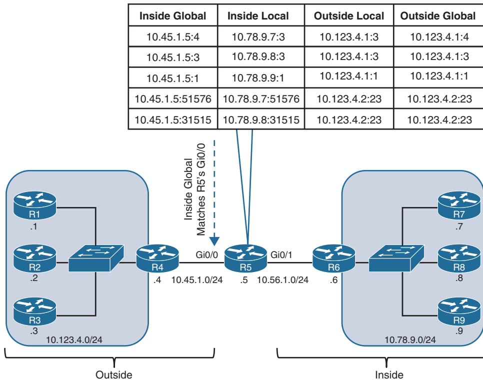
Figure 15-10 R5's Translation Table for PAT
