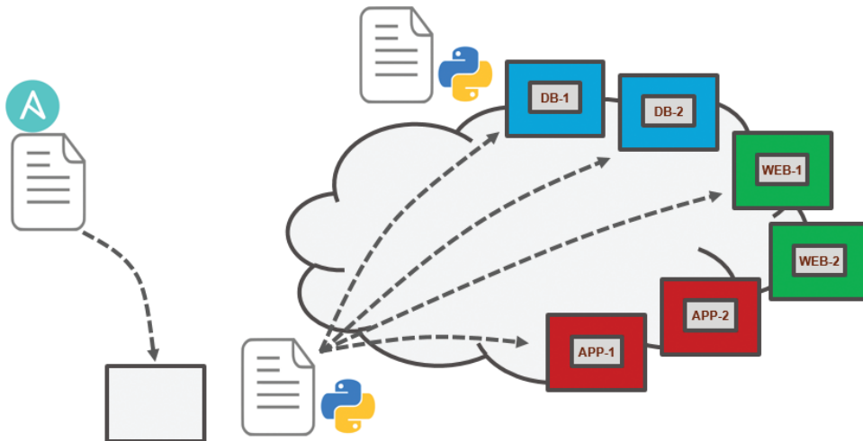
Figure 29-8 Ansible Workflow
