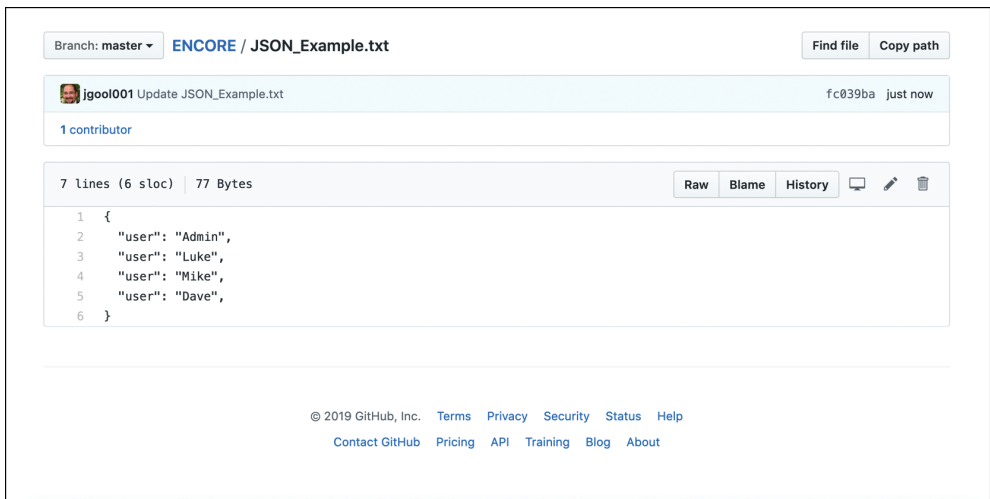
Figure 28-22 JSON_Example.txt Contents
