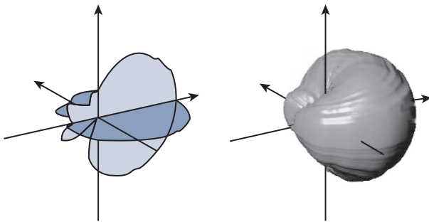
Figure 18-21 Patch Antenna Radiation Pattern in Three Dimensions
