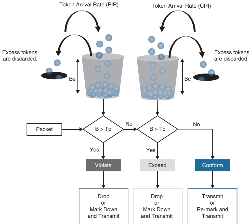
Figure 14-16 Two-Rate Three-Color Marker/Policer Token Bucket Algorithm
