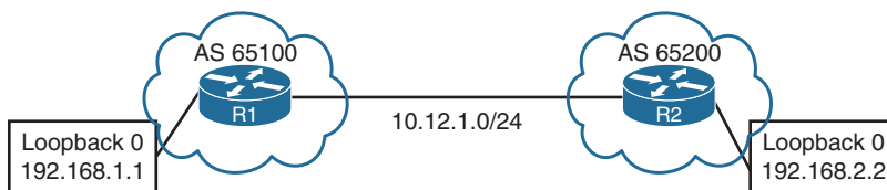
Figure 11-7 Simple BGP Topology
