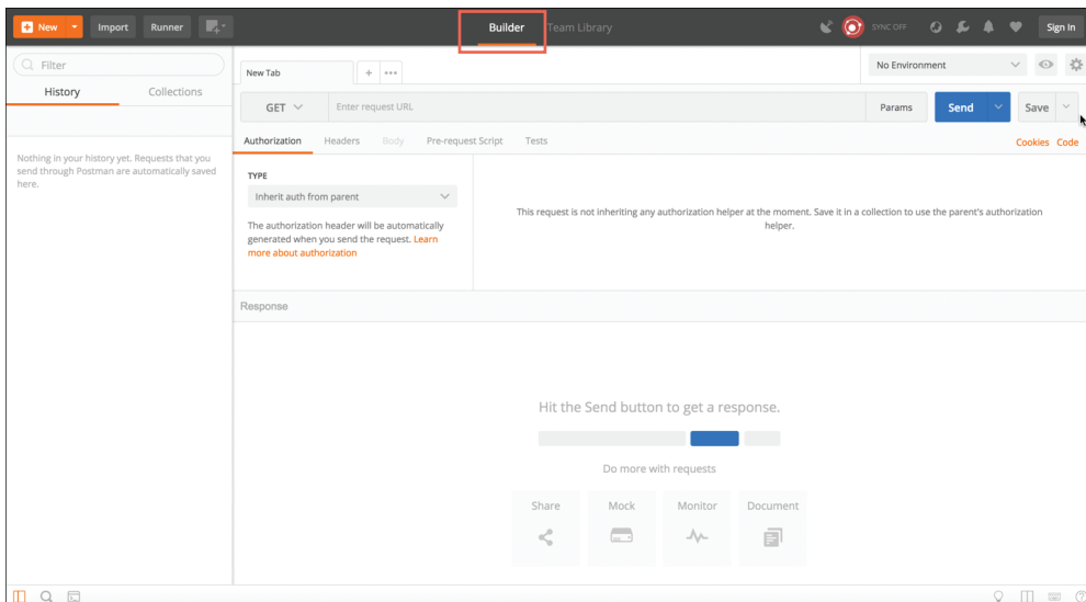
Figure 28-2 Postman Dashboard
