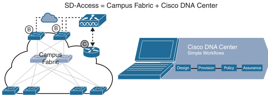
Figure 23-1 SD-Access Solution
