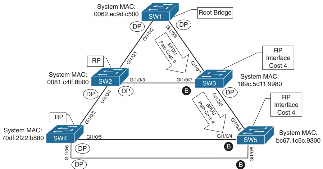
Figure 3-2 STP Path Cost Calculation
