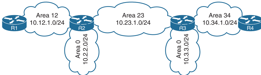
Figure 9-12 Discontiguous Network
