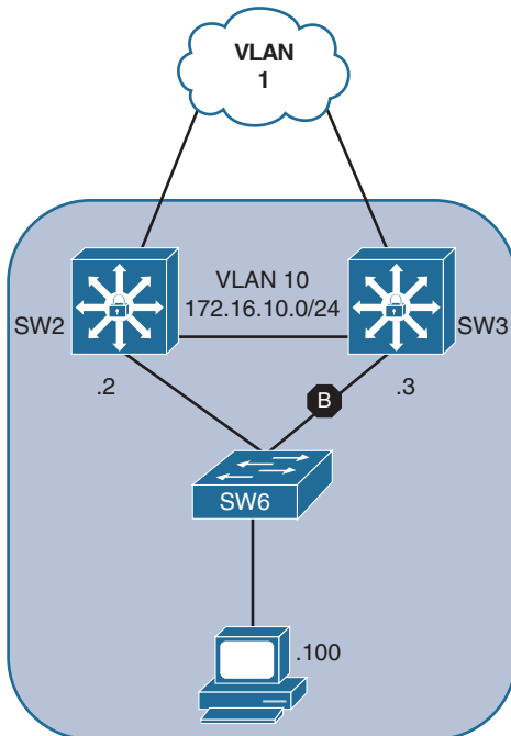
Figure 15-6 Sample HSRP Topology
