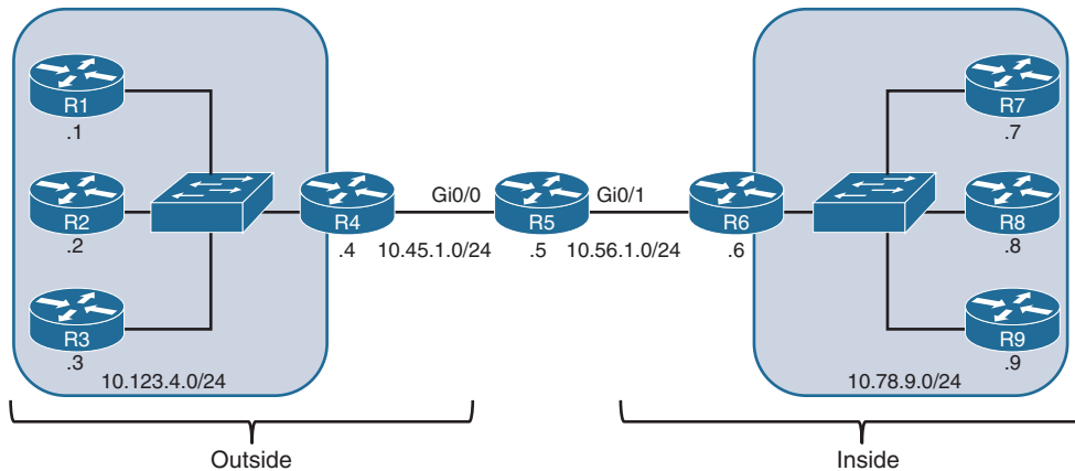
Figure 15-7 NAT Topology
