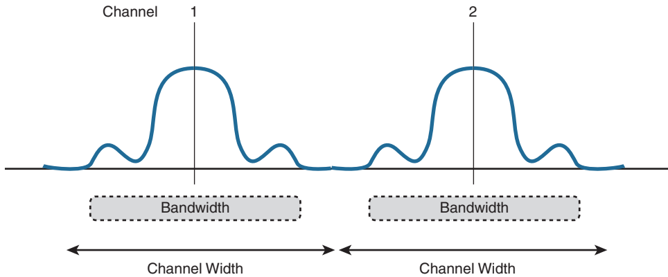
Figure 17-9 Non-overlapping Channel Spacing
