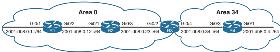
Figure 10-1 OSPFv3 Topology
