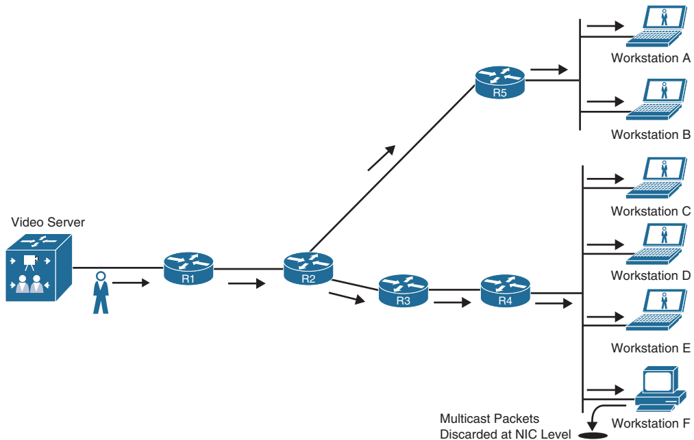
Figure 13-4 Multicast Video Feed
