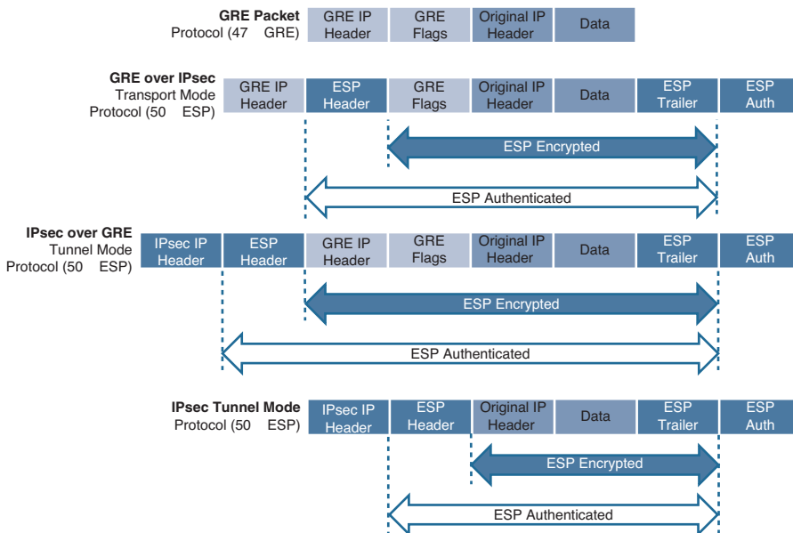
Figure 16-4 GRE over IPsec Versus IPsec Tunnel Mode
