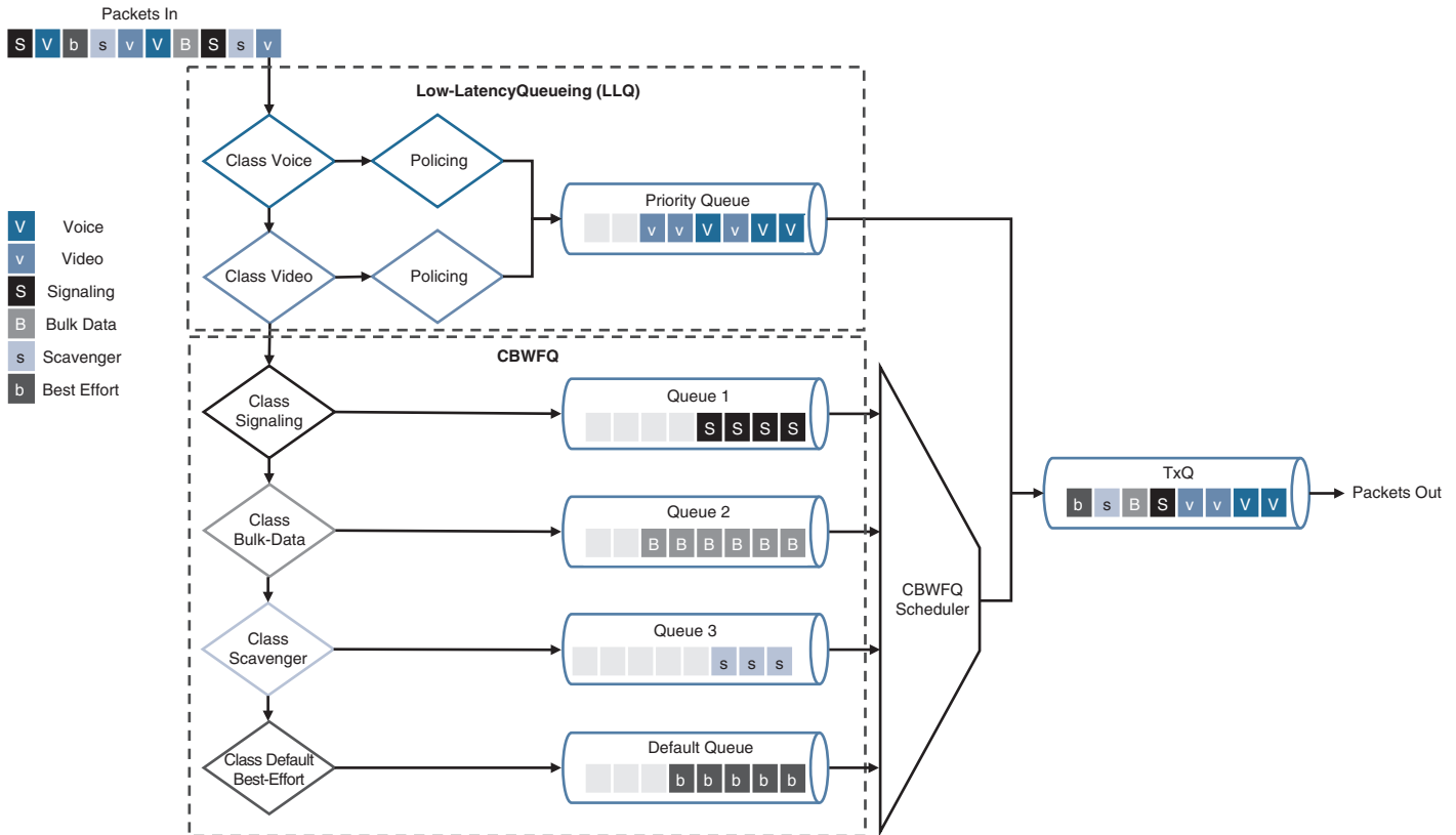
Figure 14-17 CBWFQ with LLQ
