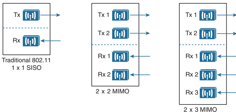
Figure 17-28 Examples of SISO and MIMO Devices
