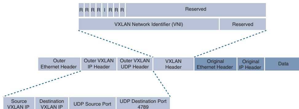
Figure 16-13 VXLAN Packet Format
