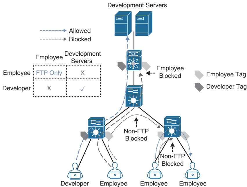
Figure 25-17 SGACL Enforcement Scenario
