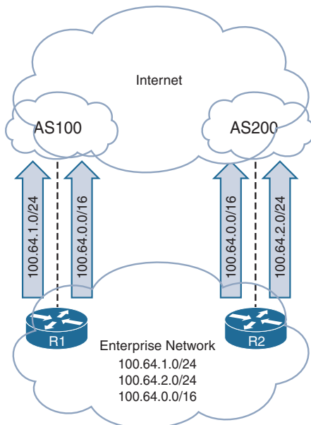
Figure 12-10 BGP Path Selection Using Longest Match
