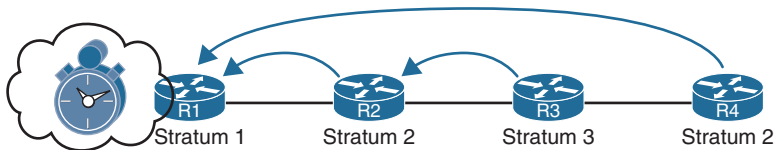
Figure 15-1 NTP Stratums
