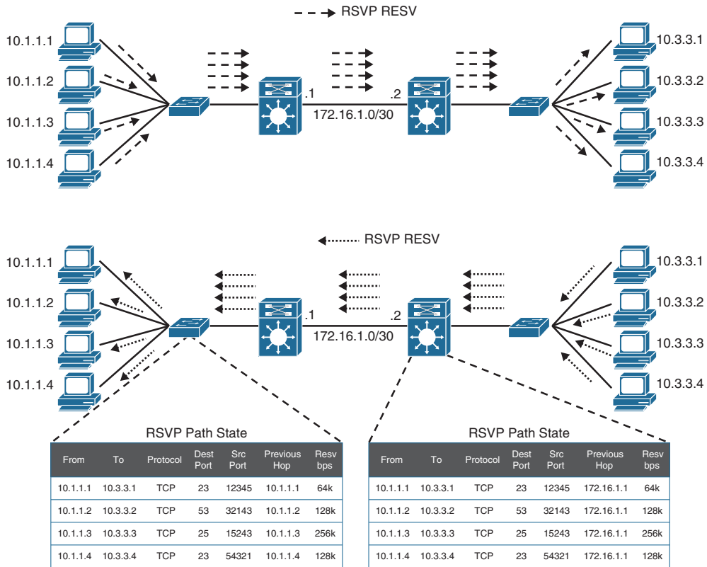
Figure 14-1 RSVP Reservation Establishment
